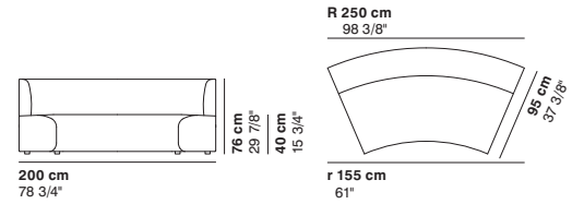
cod. 9018 / closed element curved 200
