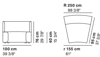
cod. 9016 / closed element curved 100
