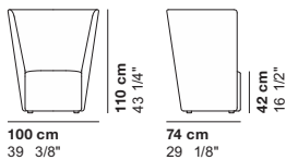
cod. 3500 / B_armchair with feet H.110
