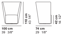
cod. 3501 / B_swivel armchair H.110
