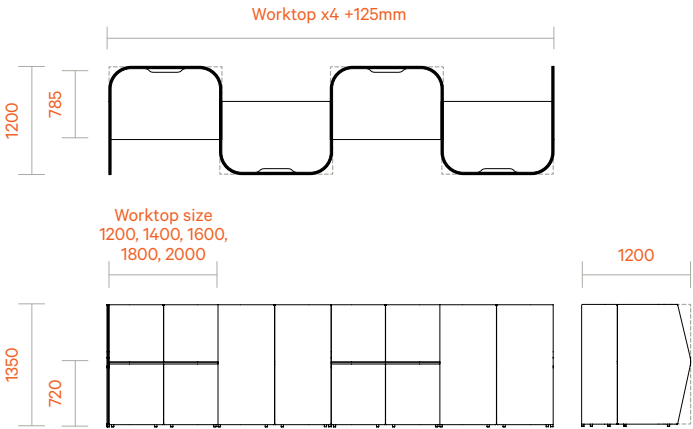
Glide detail
