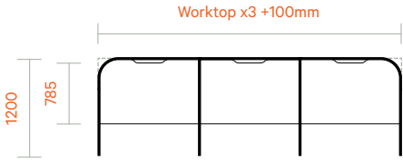
Worktop size 1200, 1400, 1600, 1800, 2000
