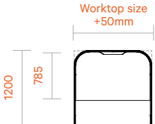
Worktop size 1200, 1400, 1600, 1800, 2000
