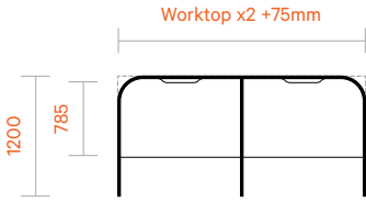
Worktop size 1200, 1400, 1600, 1800, 2000
