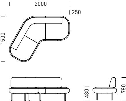
BL120E-20 120° Angle - Back Centred
