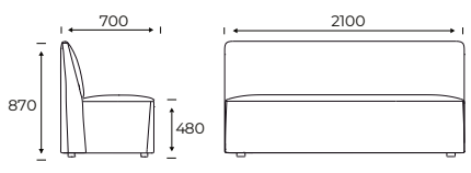
FourLikes®, Low Back, 2100
