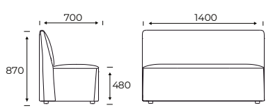
FourLikes®, Low Back, 1400
