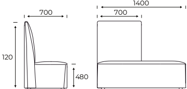
FourLikes®, Open End Left, High Back Right, 1400
