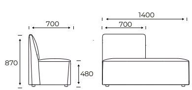
FourLikes®, Open End Left, Low Back Right, 1400
