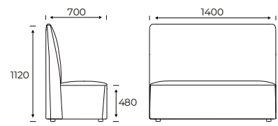
FourLikes®, High Back, 1400
