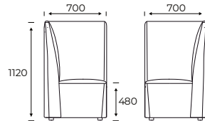
FourLikes®, Corner, High Back, 700
